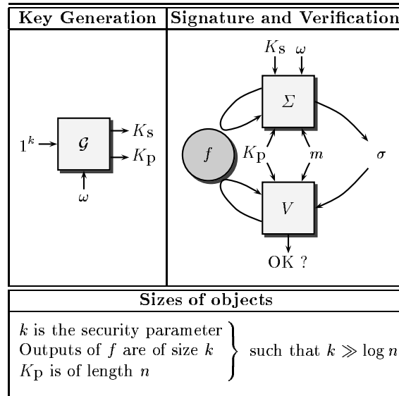
Fig. 1. Signature schemes.
