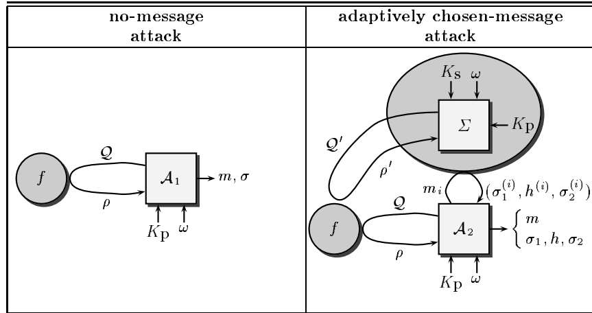
Fig.2. Attacks.
