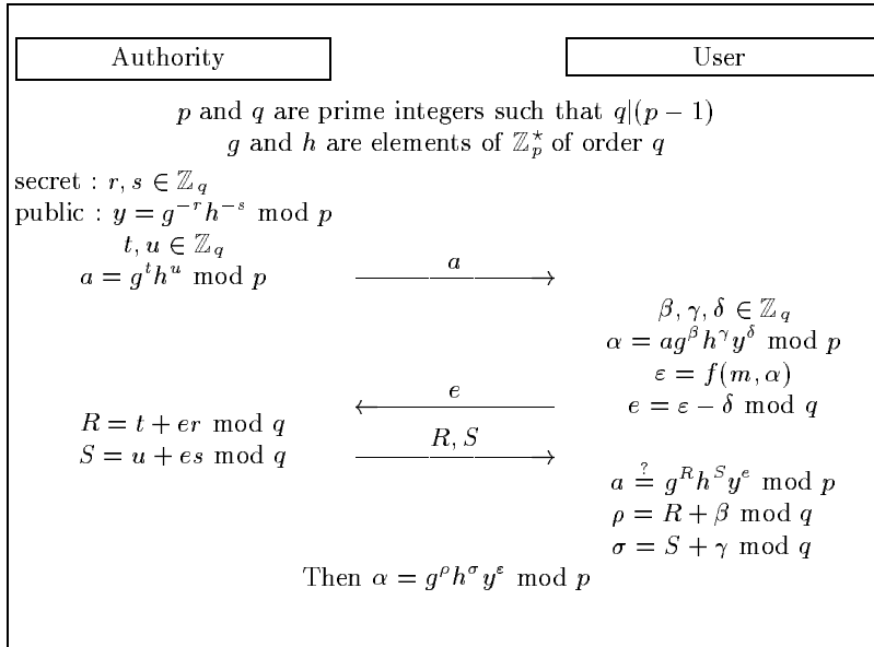
Fig. 11. The Okamoto-Schnorr blind signature scheme
