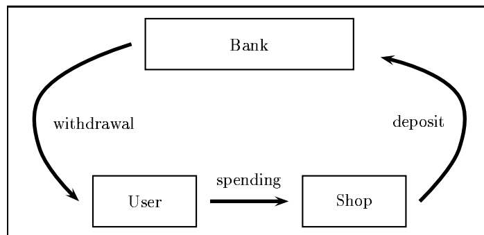
Fig. 3. Coin life.
