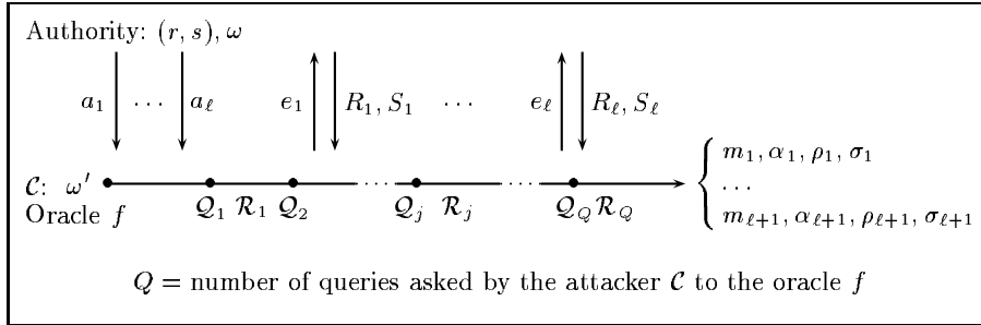
Fig. 5. The parallel attack.
