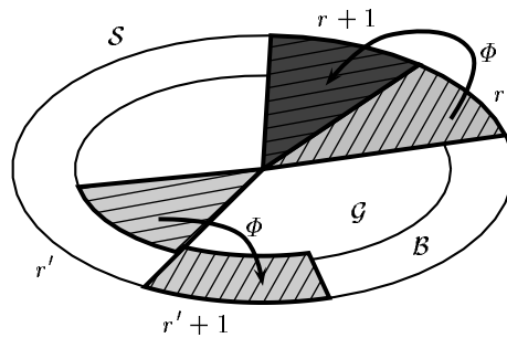
Fig. 13. Properties of \Phi .
