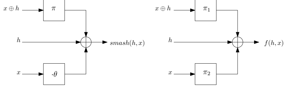
Fig. 1. SMASH compression function and our 2-permutation based compression function.
