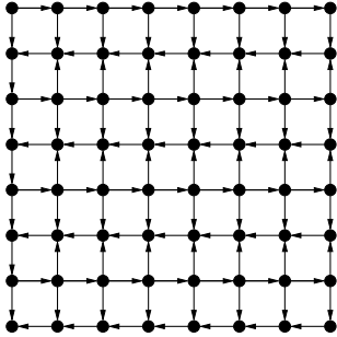
Figure 2. The directed grid \mathcal{S}_8^d
