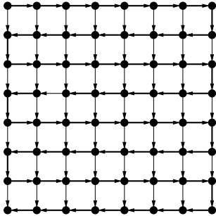
Figure 2. The directed grid S_8^d
