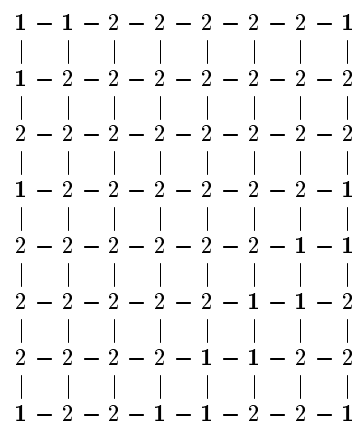
(a) The colored grid \mathcal{S}_8
