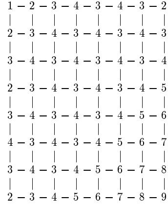
(b) The colored grid \mathcal{S}'_8
