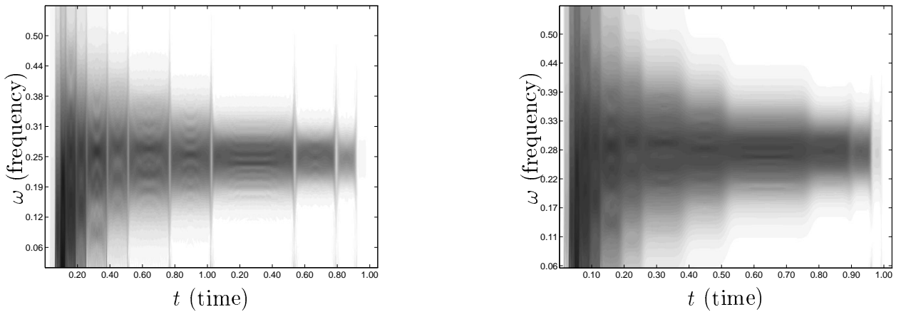
FIG. 9. The left image is the estimated time-varying power spectrum \tilde{\Lambda}_0(t, \omega) in the best local cosine basis. The right image displays \hat{\Lambda}_0(t, \omega) computed in the same best basis, with modified maximally smooth windows.
