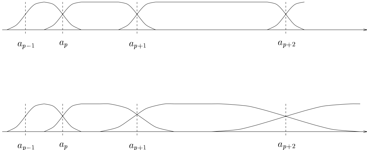
FIG. 7. The figure at the top gives an example of windows for a local cosine basis. The figure at the bottom shows how to dilate the rising and decaying profiles to obtain windows of maximum smoothness, while maintaining the necessary properties for local cosine bases.
