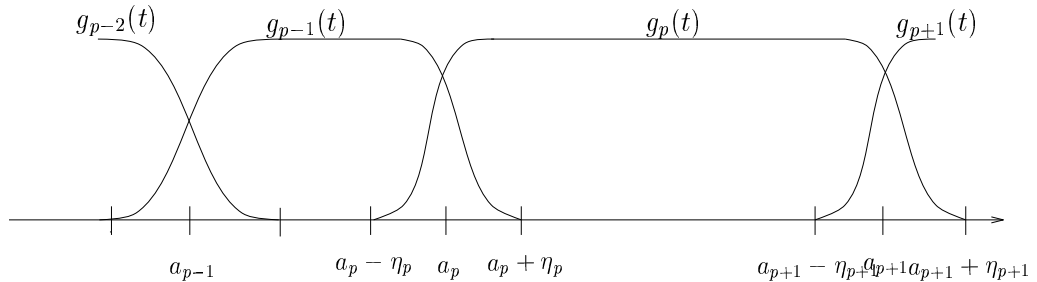
FIG. 2. Smooth cutoff window functions g_p(t) , p \in \mathbf{N} , used in local cosine bases. The supports of adjacent windows g_p(t) and g_{p-1}(t) intersect over the interval [a_p - \eta_p, a_p + \eta_p] . Over this interval, both windows are symmetric with respect to a_p .
