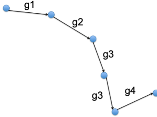
FIGURE 14 – Illustration de la notion de transport.
