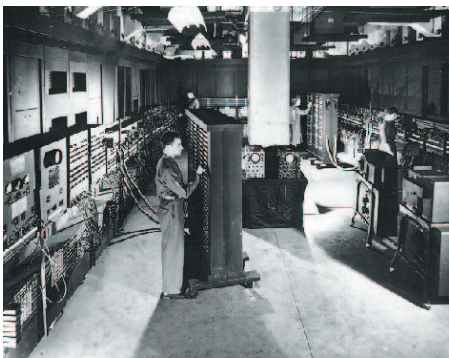
ENIAC 5,000 flops 3
