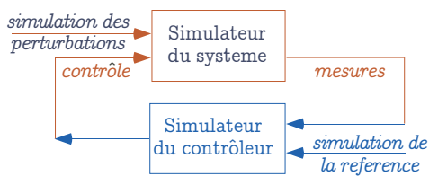
(2) Simulation
