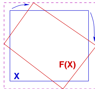
X \cup F(X) intervalle instable
