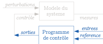
(3) Implantation
