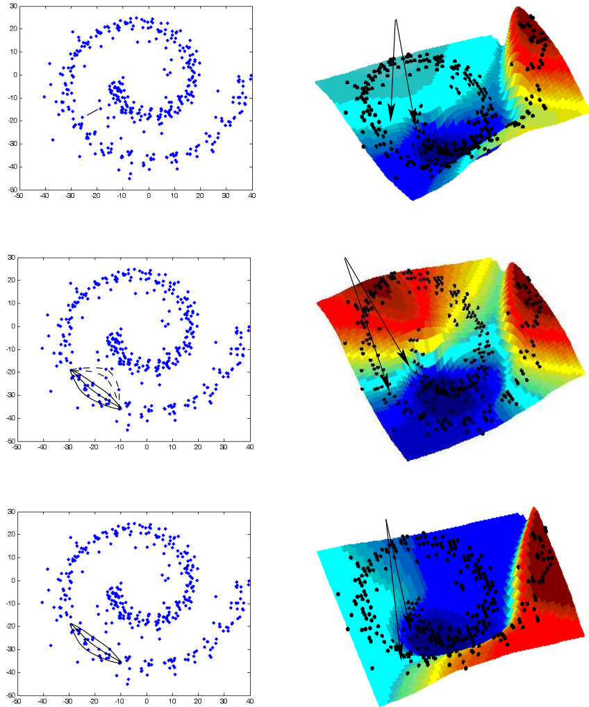
FIG. 2 – The left figures show samples taken from the Swiss roll. (top) A short cut makes the random walk Laplacian embedding very noise sensitive, clearly the variation of the color map does not follow the intrinsic dimension of the actual manifold. (middle) When using the diffusion map, noisy paths affect the estimation of the conditional probabilities. This issue is overcome in (bottom) when using the robust diffusion map, as now the color map varies following the intrinsic dimension.
