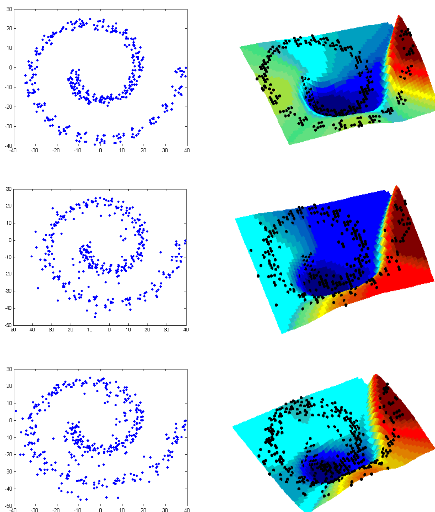
FIG. 3 – Robustness of the embedding with respect to uniform noise throughout the curvilinear abscissa of the Swiss roll. From top to bottom, the noise is 0%, 15% and 40%.
