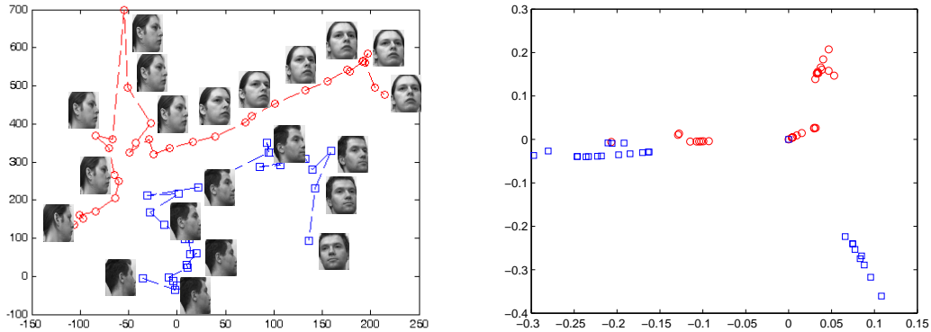
FIG. 1 – (Left) This figure shows the distribution of two classes corresponding to two individual. It is clear that the intra class variance is larger than the inter class one. (Right) This is the distribution of the same classes inside the manifold trained using graph Laplacian. It is clear that the converse is now true and the classification task is easier in the embedding space.
