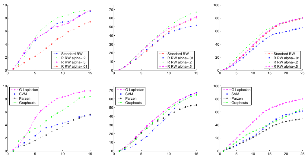
FIG. 5 – (Top) These figures show the recall for Orl , Swedish and Corel databases for different graph Laplacians. (Bottom) Comparison of Graph Laplacian with respect to SVM, Parzen and Graph-cuts.
