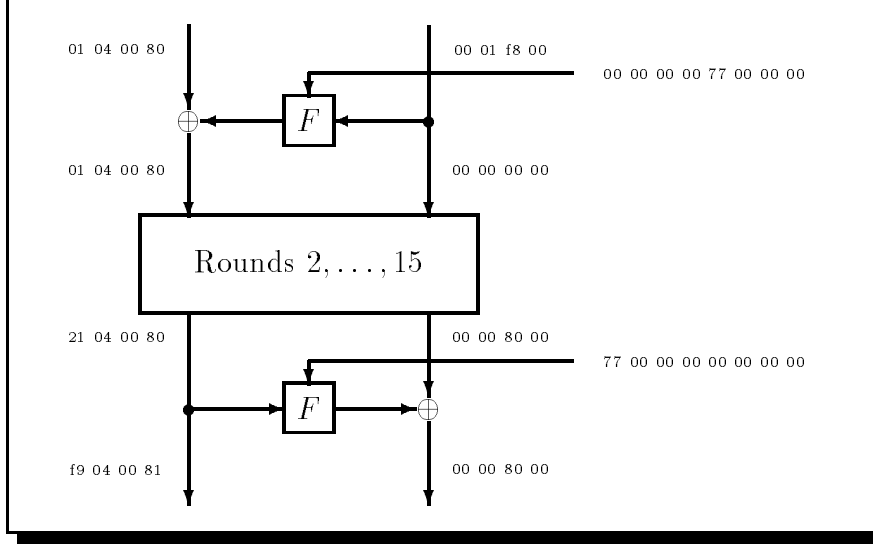
Figure 3: Matsui's characteristic
