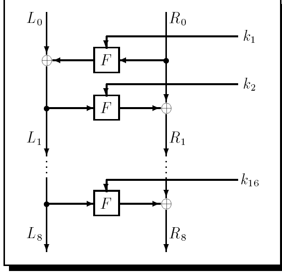
Figure 1: Feistel's scheme with 16 rounds
