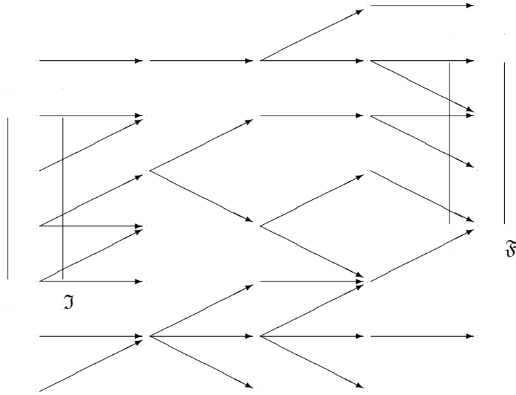
FIGURE 10. Descendant states ( \bullet ) of the initial states ( \mathcal{J} ).
