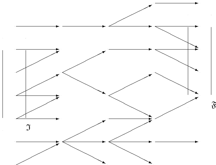
FIGURE 11. Ascendant states ( \bullet ) of the final states ( \mathfrak{F} ).
