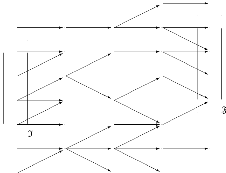
FIGURE 12. Descendant states ( \bullet ) of the initial states ( \mathcal{J} ) which are ascendant states of the final states ( \mathcal{S} ).
