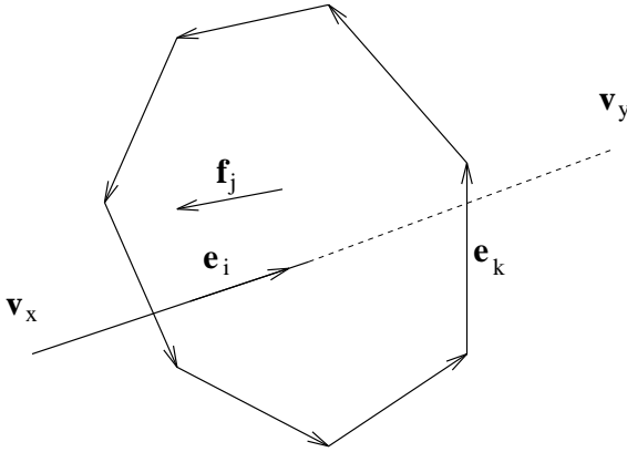
Fig. 6. Basic edge-face intersection test (convex faces).
