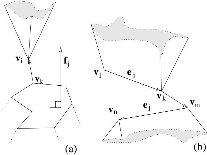
Fig. 5. Geometric elements involved in the definition of the predicates associated with Type-A (a) and Type-B (b) basic contacts.
