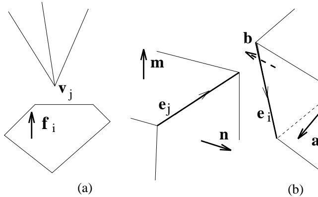
Fig. 18. (a) An applicable vertex ( V_j ) - face ( F_i ) pairing. (b) Edges E_i and E_j are also applicable.
