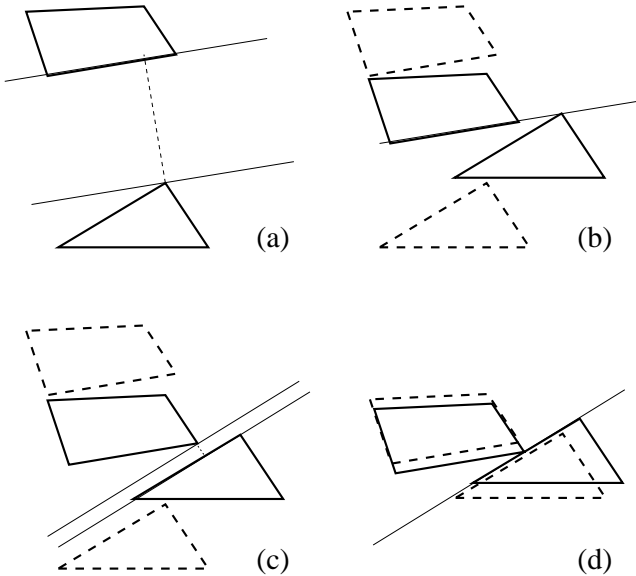
Fig. 9. Adaptive time sampling. Starting position is depicted in (a), where the closest points and the line joining them are computed. The projections of the objects on this line meet at instant (b), which is taken as the next time sample. At this instant, the new closest points are computed (c), and the next time sample, where the polygons do actually collide, is determined in the same way (d).
