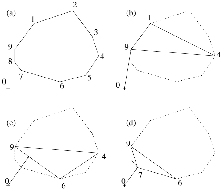
Fig. 14. The closest point of the original Minkowski polygon (a) to the origin ( 0 ) has to be determined. The first simplex (b) has been chosen arbitrarily. A subset of vertices, whose convex hull contains the closest point of the simplex to the origin, is taken (4 and 9, although in this case also 1 and 9 could have been chosen), and a new vertex is selected (c). Note that this new vertex, 6, has the minimum projection onto the direction to the closest point found in (b). At the same time, the non-relevant vertex 1 is deleted. The direction to the closest point of the simplex in (c) is computed, and in the next step the closest point of the polygon to the origin (7 in this case) is determined (d).
