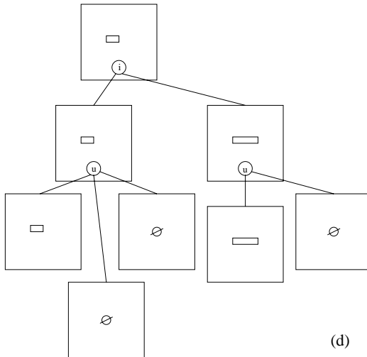
Fig. 2. S -bounds (cont.). (c) The box obtained at the root node is intersected with the boxes of nodes at lower levels. The empty set is obtained for some nodes, which can be eliminated. (d) The representation is once again explored upwards, and a smaller box is obtained at the root. If the process is repeated once more every node will contain the small box or the empty set. This small box bounds the region where intersection has to be looked for.
