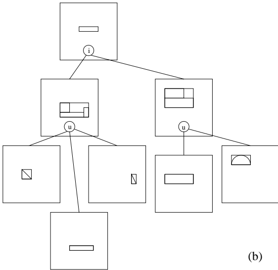
Fig. 1. S -bounds. (a) The intersection ( i ) between two polygons described by their CSG representations has to be computed. (b) The rectangular boxes that bound the primitives are combined and the boxes corresponding to the higher levels are determined, according to the nature of the nodes (union or intersection).
