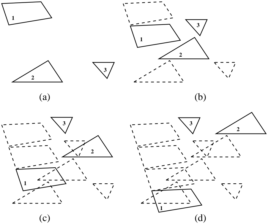
Fig. 8. Multiple interference detection approach. As the time step is too large, the collision between the polygons 1 and 2, which takes place between instants (b) and (c), is missed. At instant (d) polygons 1 and 2 have attained their final positions, whereas polygon 3 had already attained it between instants (b) and (c). The polygons and their trajectories are the same as those in the next three figures.
