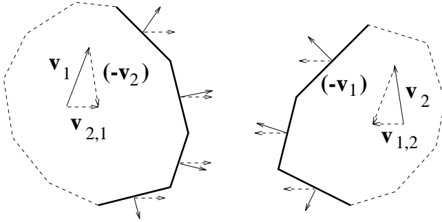
Fig. 17. Only the faces (shown as heavy lines) whose normals have positive projections on the relative motion vectors ( v_{2,1} and v_{1,2} ) need to be considered.
