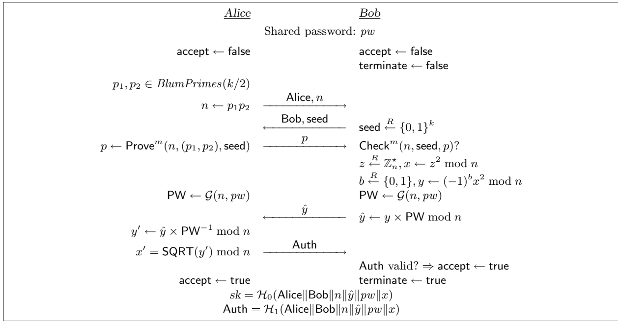
Fig. 2. SQRT – IPAKE protocol
