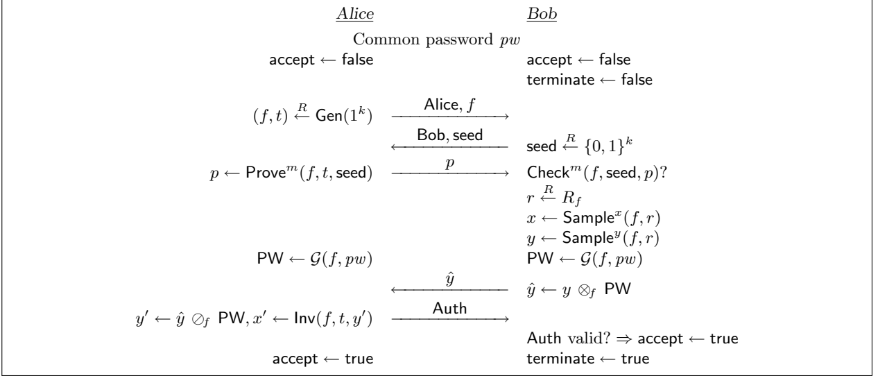
Fig. 1. An execution of the IPAKE protocol: Auth is computed by Alice (Bob resp.) as \mathcal{H}_1(\text{Alice}||\text{Bob}||f||\hat{y}||pw||x) ( \mathcal{H}_1(\text{Alice}||\text{Bob}||f||\hat{y}||pw||x') resp.), and sk is computed by Alice (Bob resp.) as \mathcal{H}_0(\text{Alice}||\text{Bob}||f||\hat{y}||pw||x) ( \mathcal{H}_0(\text{Alice}||\text{Bob}||f||\hat{y}||pw||x') resp.)
