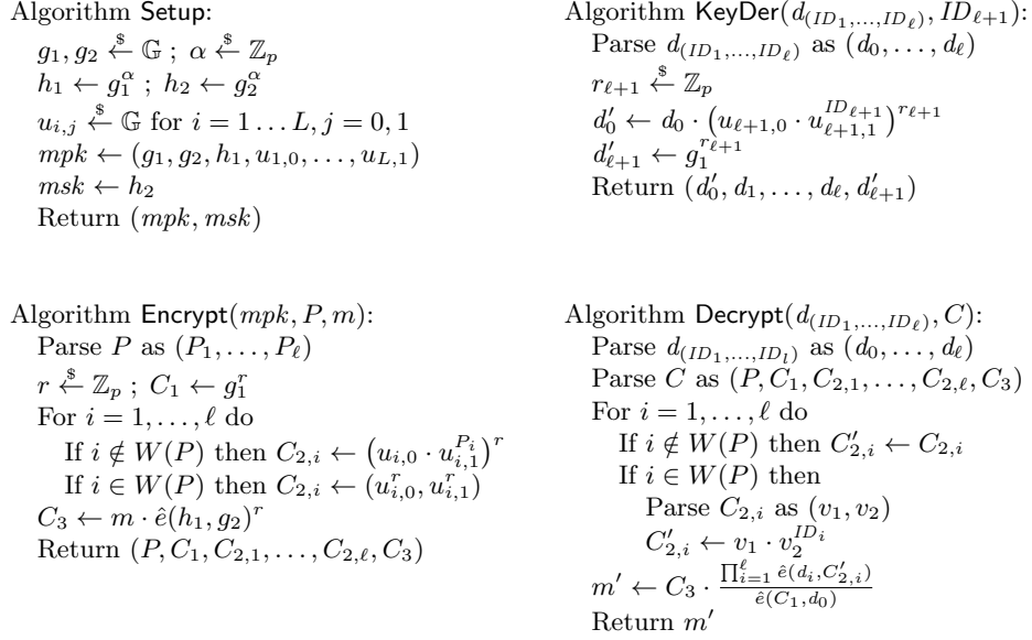
Fig. 4. The Boneh-Boyen WIBE scheme.
