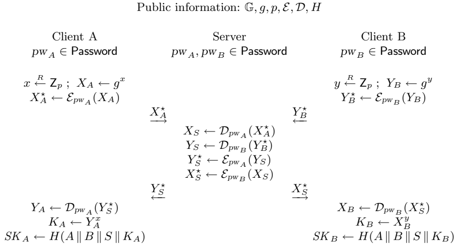
Fig. 1. A 3-party password-based encrypted key exchange protocol that is insecure against insider attacks. \mathcal{E}_{pw} and \mathcal{D}_{pw} represent, respectively, the encryption and decryption algorithms of a cipher, such as AES [3], using the password pw as the encryption and decryption key.
