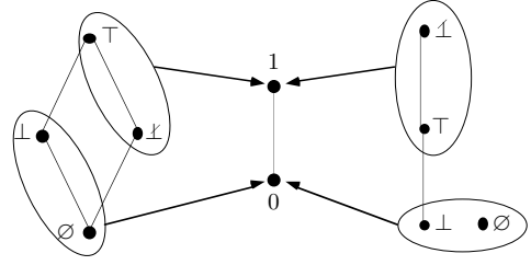
Figure 3: Abstraction of the basic compartment approximation and computation orderings into Mycroft's strictness ordering
