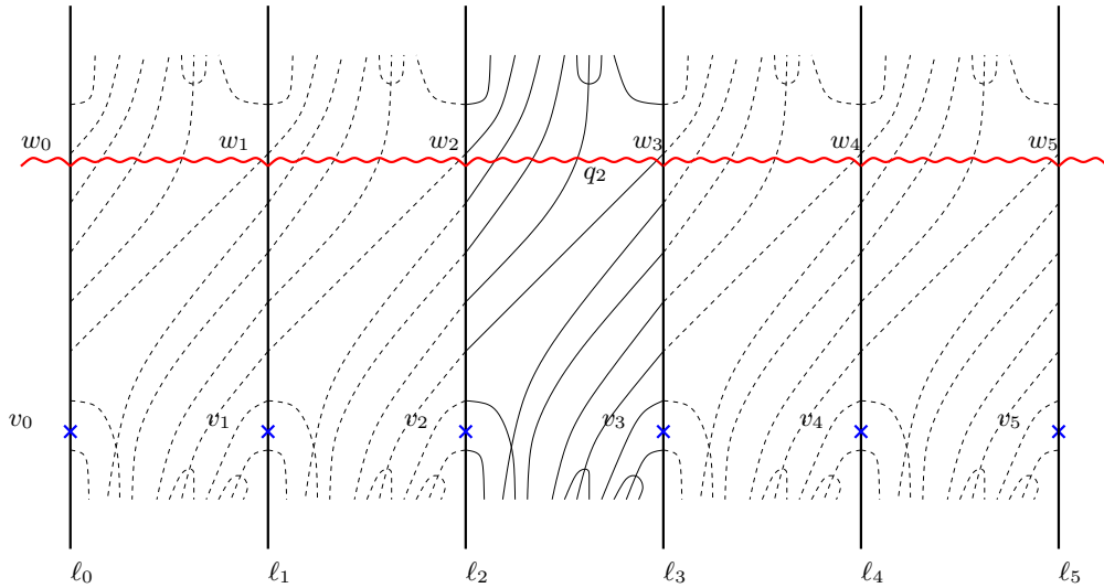
Figure 10. The part of the universal cover containing the lifts of \gamma and \delta , and the lines \ell_i . Other lines in this area are also shown.
