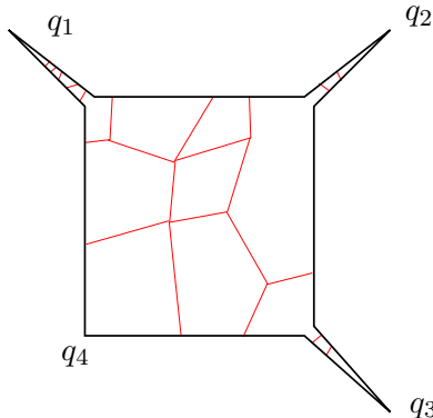
Figure 11. A polygonal schema and the sub-edges. The internal sub-edges have both endpoints on the boundary of the polygonal schema, while the external sub-edges have at least one endpoint at a vertex of G^* .
