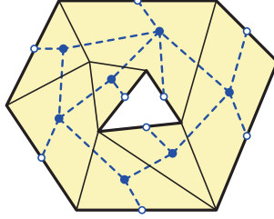
Figure 1. Primal (solid) and dual (dashed) graphs on a combinatorial annulus.
