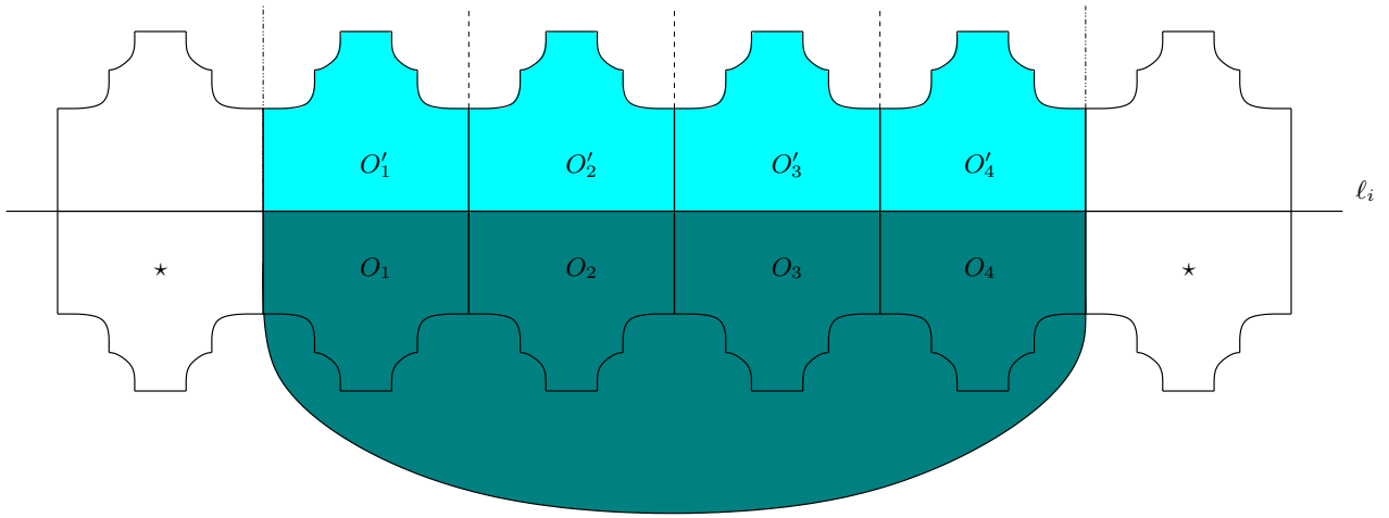
Figure 8. From \tilde{\mathcal{M}}_{i-1} (dark shaded) to \tilde{\mathcal{M}}_i (all shaded).
