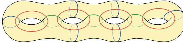
Figure 2. An octagonal decomposition built by our algorithm.
