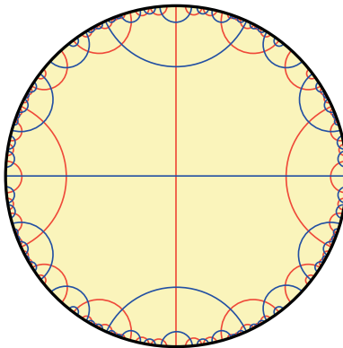
Figure 7. Universal cover of an octagonal decomposition.
