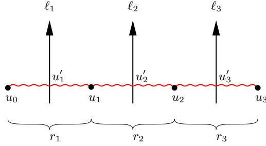
Figure 9. The notations for the proof of Lemma 4.6.
