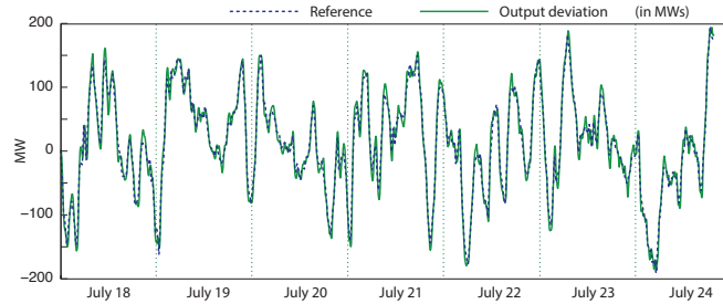
Fig. 10. Closed loop simulation with Markovian model.
