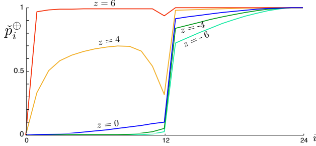
Fig. 6. Transformed probability vector \check{p}^\oplus under \check{P} .
