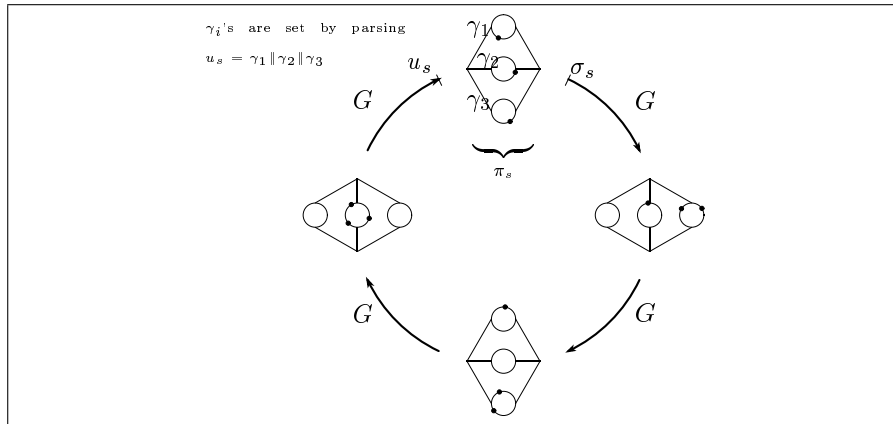
Fig. 3. The ring composition paradigm. Here we have t = 3 . If \pi_s is a fair partition w.r.t. three signers, they start from a seed \sigma_s and compute u_s . Finally they solve the sub-rings in \pi_s according to the obtained gaps \gamma_1, \dots, \gamma_3 . The equation is verified in a straightforward way, starting at any given index.
