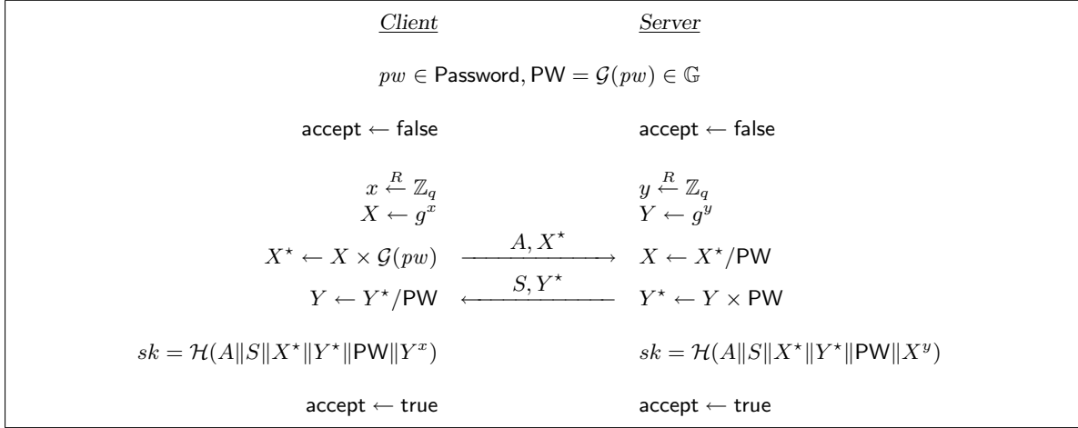
Fig. 5. An execution of the protocol MDHKE.
