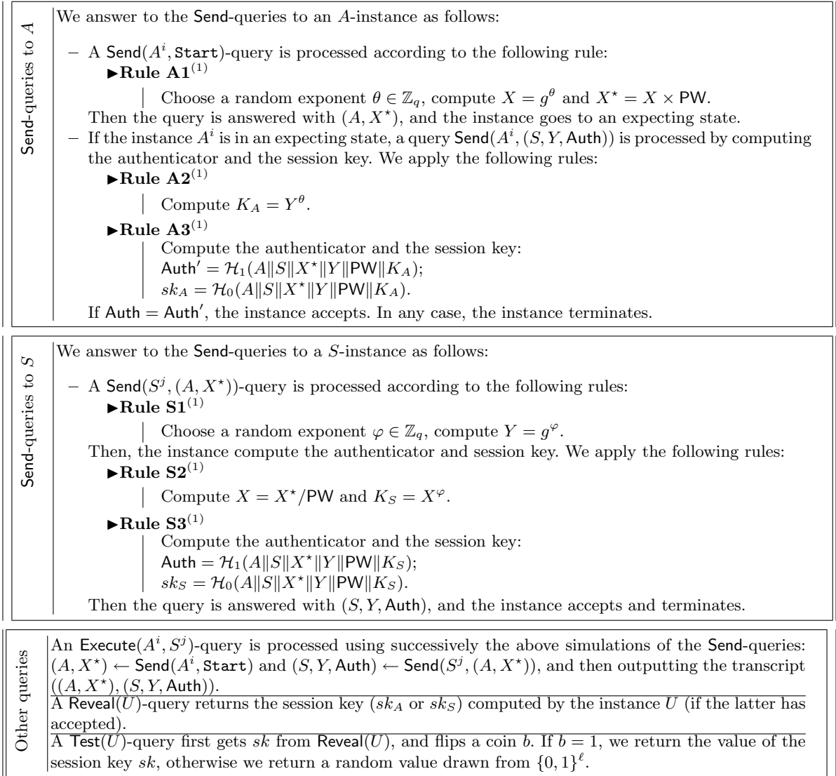
Fig. 3. Simulation of the OMDHKE protocol
