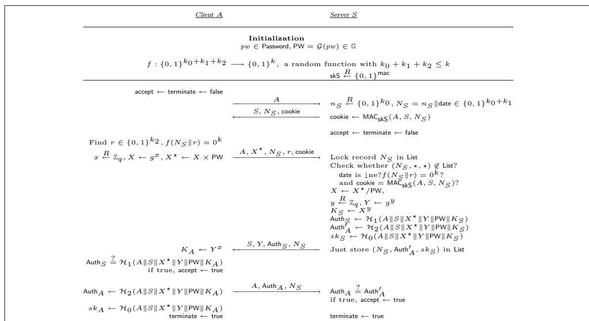
Fig. 4. An execution of the protocol OMDHKE, run between a client and a server, enhanced with mutual authentication and a denial-of-service protection.
