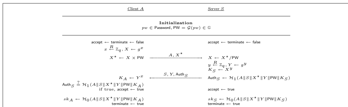
Fig. 1. An execution of the protocol OMDHKE, run between a client and a server.
