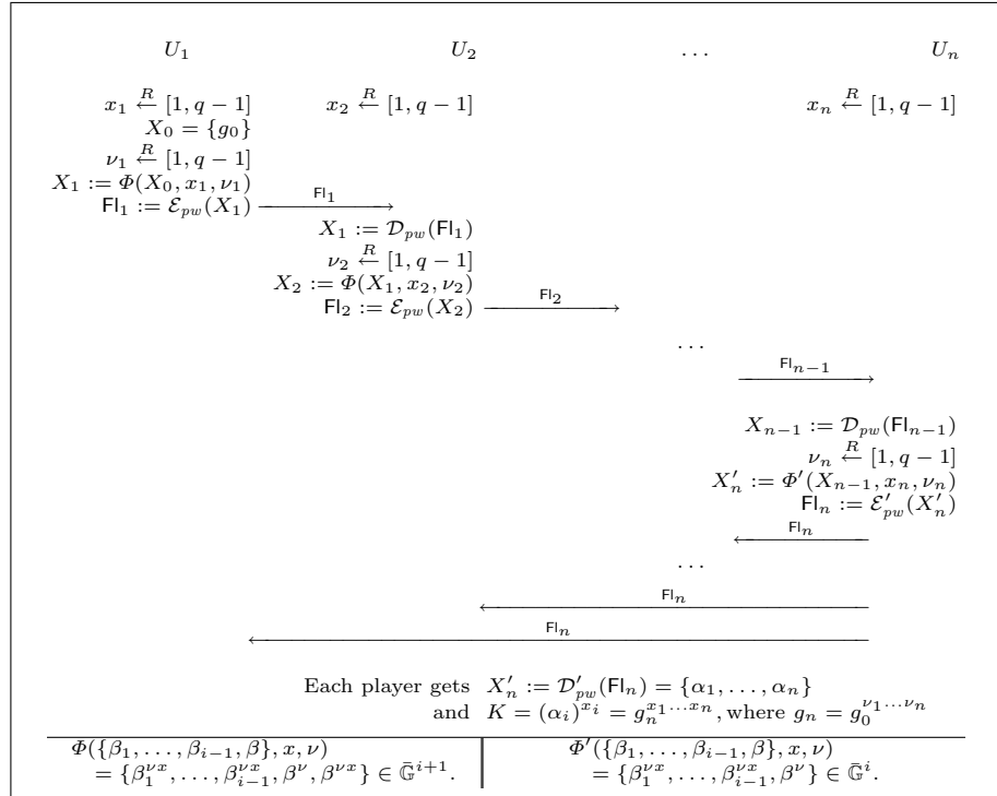
Fig. 2. Protocol EKE. The multicast group is \mathcal{U} = \{U_1, U_2, \dots, U_n\} and the session key is sk = \mathcal{H}(\mathcal{U} \parallel \text{Fl}_n \parallel K) .
