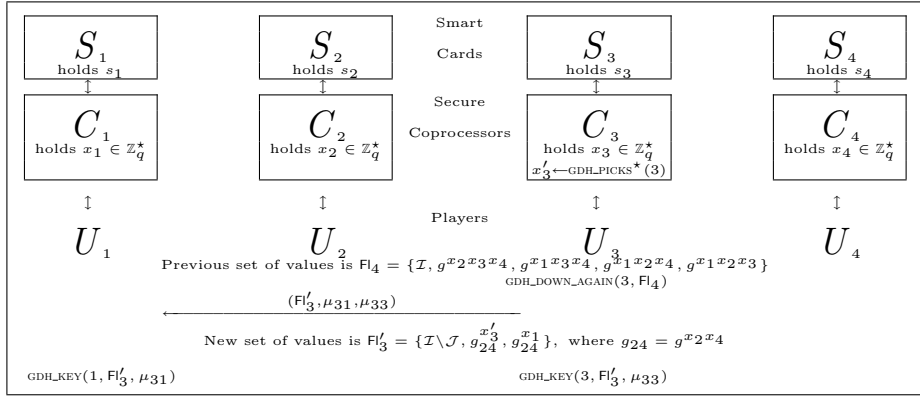
Fig. 2. Algorithm Remove1 + . A practical example with 4 players: \mathcal{I} = \{U_1, U_2, U_3, U_4\} and \mathcal{J} = \{U_2, U_4\} . The new multicast group is \mathcal{I} = \{U_1, U_3\} and GC = U_3 .
