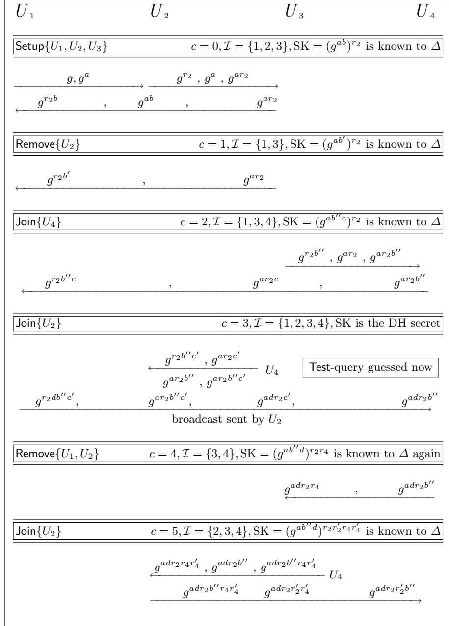
Fig. 7. An example of an execution of the protocol P=\text{AKE1} with the adversary. We represent the simulation by \Delta according to the following “guesses”: c_0 = 3, s = 4, \mathcal{I}_0 = \{1, 2, 3, 4\}, i_0 = 2 . We denote by b, b', b'' etc. some blinding exponents used in the self-reduction of G-CDH (think b'' as being b\beta'' , e.g.). Also note that when rejoining the group at steps c = 3 and c = 5 , U_2 does not “remove” its random exponent.
