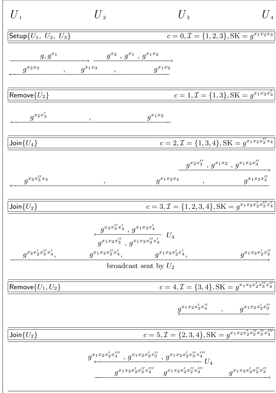
Fig. 6. An example of an execution of the real protocol P=\text{AKE1}
