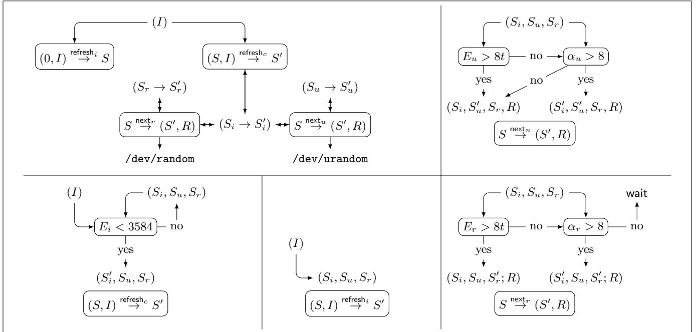
Fig. 3. Relations between functions and pools for LINUX
