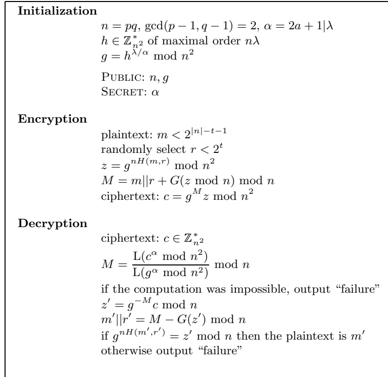
Fig. 4. Efficient variant secure against adaptive attacks (Scheme 2)
