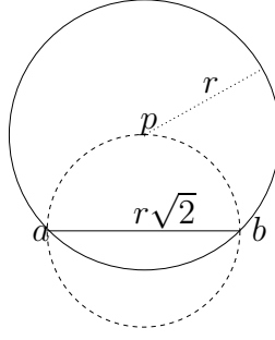
Fig. 6. The shortest shield edge ab which may be encroached upon by a rejected circumcenter p .
