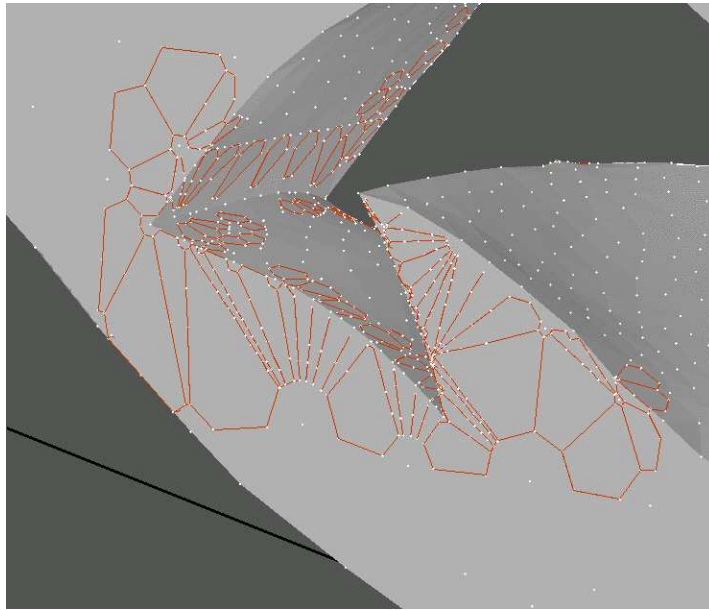
Fig. 9. Detail of a geological formation (Courtesy of T-surf and Mr. Reinsdorff). Solid line segments stand for shield edges.
