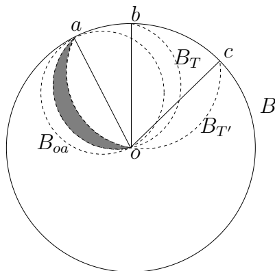
Fig. 7. \text{circum}(oab) \subset \text{circum}(oac) \cup \text{circum}(oa) .
