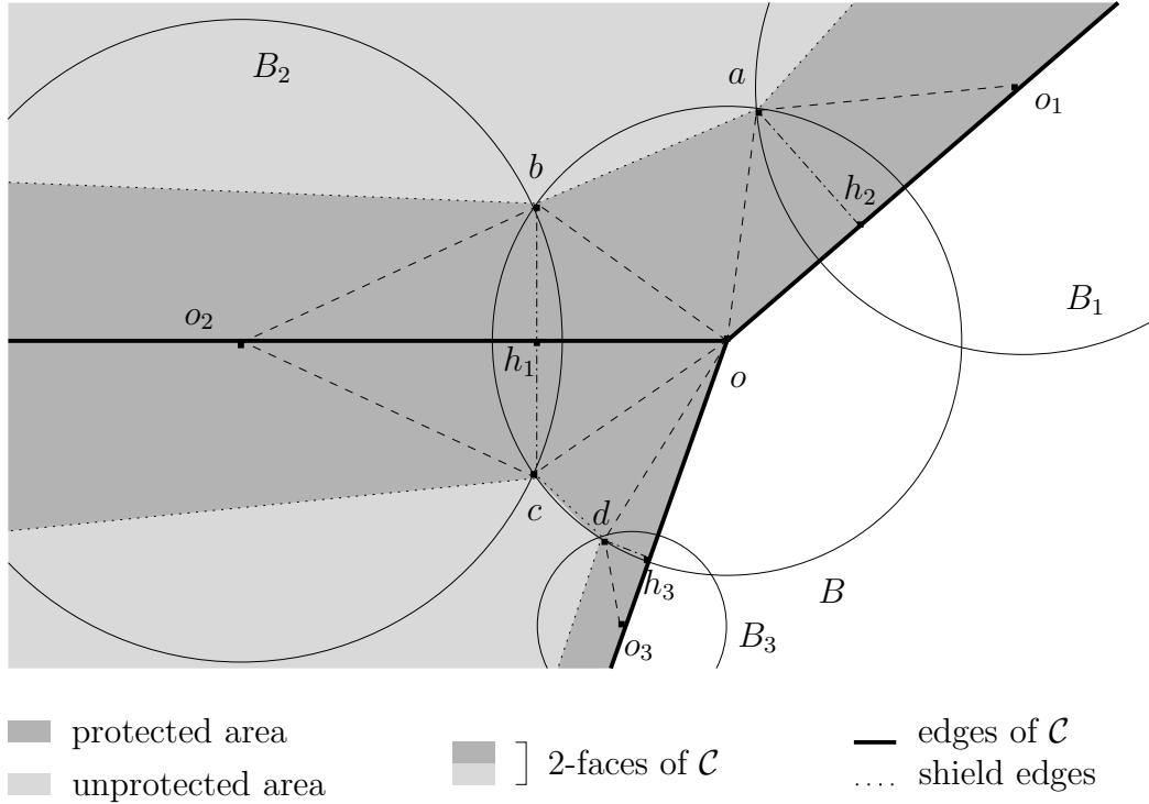
Fig. 1. The situation in the neighborhood of a ball B , incident to three other balls B_1, B_2 and B_3 . There are two faces in the complex, limited by three edges, in the plane of the figure. Point h_i is added on the radical plane of B and B_i . p -points a, b, c , and d belong to the boundary of two balls and to a face, they are therefore also inserted in \mathcal{P} . Incident to o are four right-angled triangles (e.g., oh_2a ) and two isosceles triangles (e.g., oab ). The shield edges are ab and cd .
