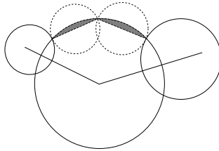
Fig. 4. The intersection of the unprotected area with the union of protecting balls is included in the circumballs of shield edges.
