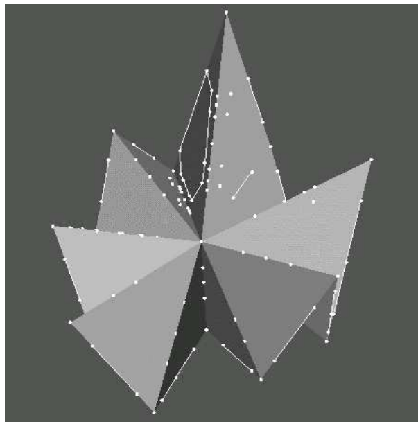
Fig. 10. Umbrella. Solid line segments stand for shield edges.
