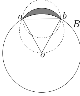
Fig. 5. The balls B , \text{circum}(oab) , and \text{circum}(ab) .
