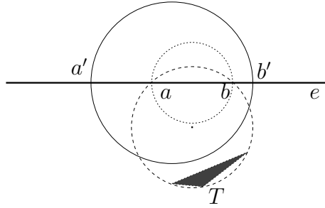
Fig. 8. In the half-space H^+ (above the edge e in the figure), the part of \text{circum}(T) is included in the part of \text{circum}(ab) which is, in turn, contained in the part of \text{circum}(a'b') .
