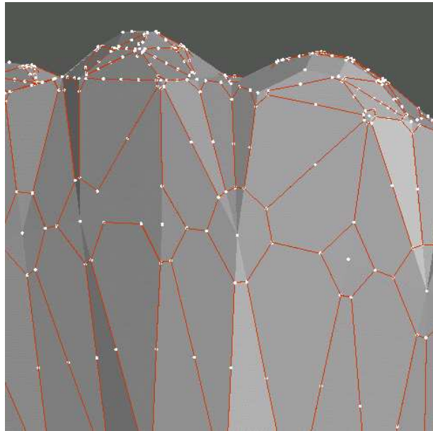
Fig. 12. Detail of the triceratops. Solid line segments stand for shield edges.
