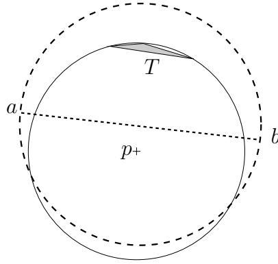
Fig. 3. The circumcenter p of a triangle T lies in the unprotected area.
