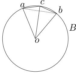
Fig. 2. The SOS strategy: We split the shield edge ab by inserting the point c on the boundary of the ball.
