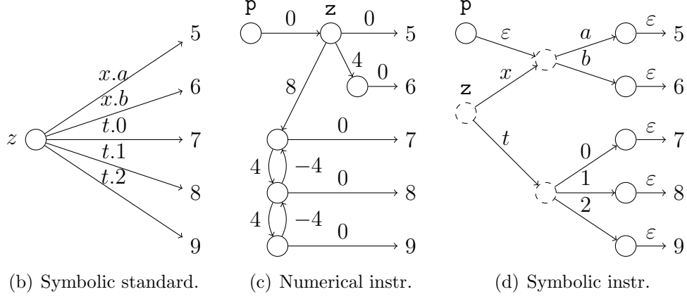
Fig. 5. Instrumented object store.
