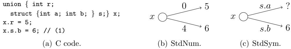
Fig. 7. Union semantics in numerical and symbolic.
