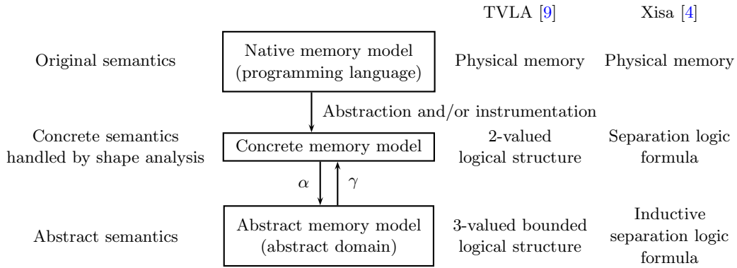
Fig. 1. Native, concrete and abstract memory models
