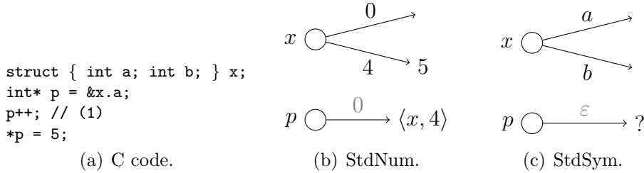
Fig. 4. Unrestricted pointer arithmetics.
