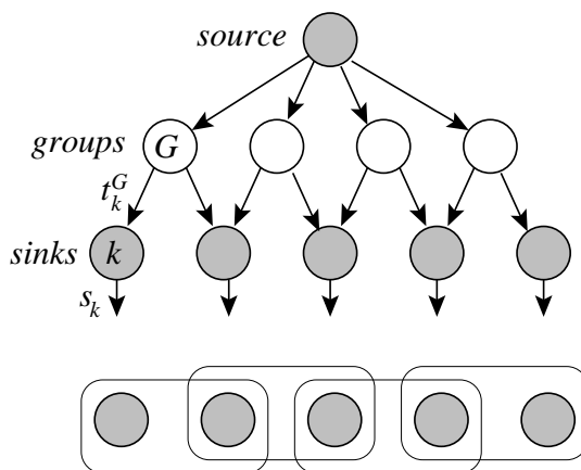
Figure 6.8: Flow (top) and set of groups (bottom) for sequences. When these groups have unit weights (i.e., D(G) = 1 for these groups and zero for all others), then the submodular function F(A) is equal to the number of sequential pairs with at least one present element. When applied to sparsity-inducing norms, this leads to supports that have no isolated points (see applications in [142]).
