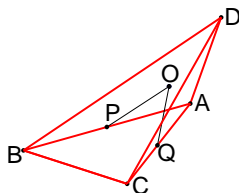
Figure 7.5: Counter-example for re-entering of a constraint in quadratic programming. We consider the problem of finding the projection of O onto the convex hull of four points in three dimensions A , B , C and D . Since O is in this convex hull, it is equal to its projection. P is the projection of O on the segment AB . Starting from the active set \{A, B\} , the best new point to add is C . The points Q is the projection of O on the triangle ABC and happens to be on the segment AC . This implies that B has exited the active set; however, it needs to re-enter in the next iteration because the optimal solution includes it.
