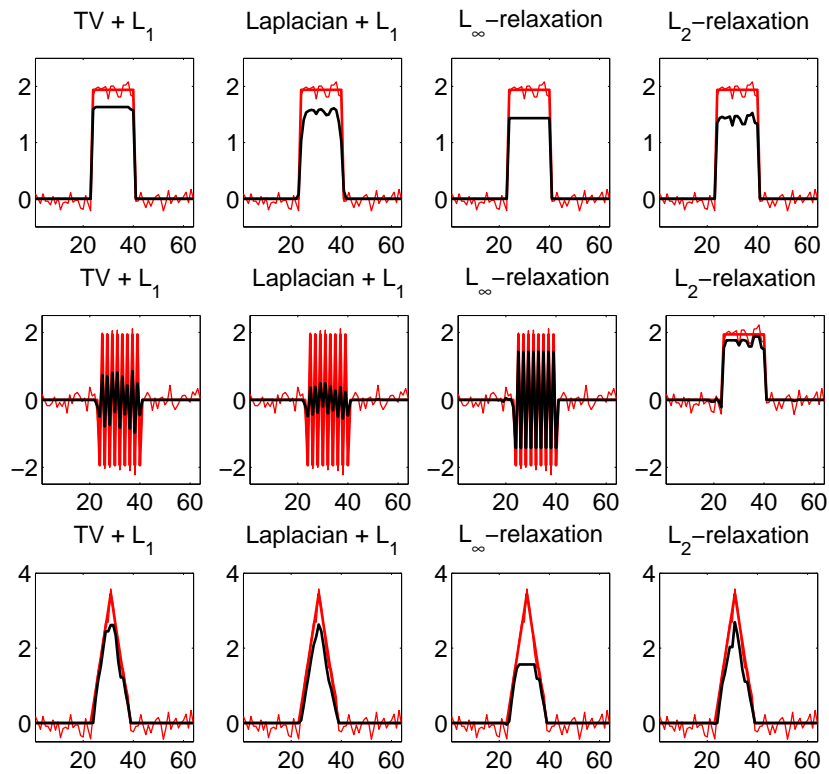
Figure 12.12: Denoising results for three different signals. Comparison of several sparsity-inducing norms. Red: signal (bold) and noisy version (plain). Black: recovered signal. See text for details.
