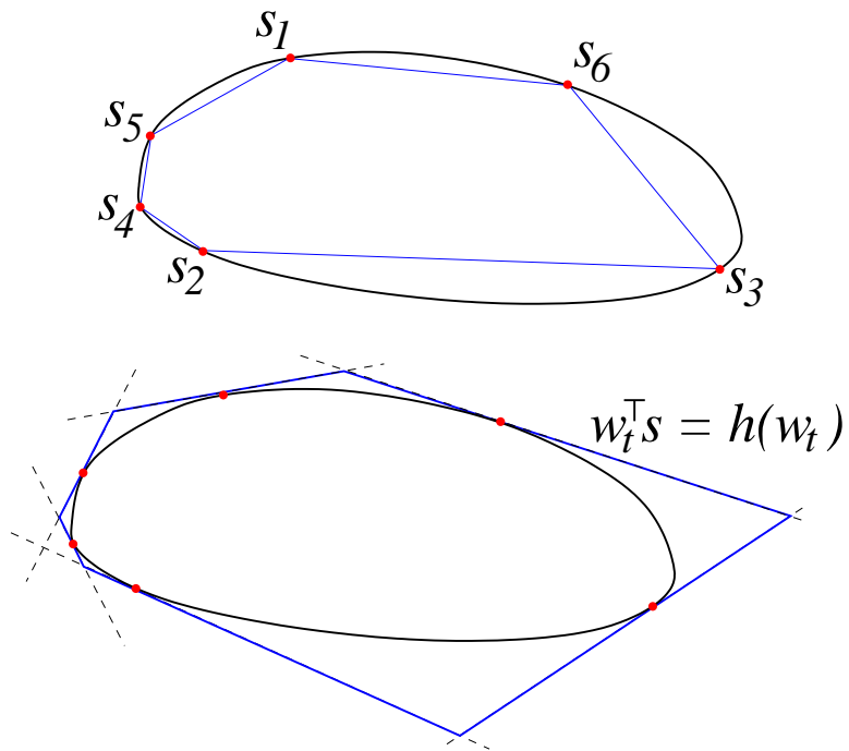
Figure 7.4: Approximation of compact convex set K : (top) inner approximation as a convex hull, used by simplicial methods in §7.7, (bottom) outer approximation as an intersection of half hyperplanes, used by dual simplicial methods in §7.8.
