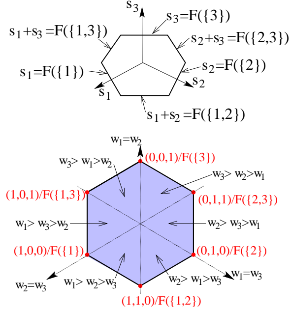
Figure 4.1: (Top) representation of B(F) for F(A) = 1_{|A| \in \{1,2\}} and p = 3 (projected onto the set s(V) = F(V) ). (Bottom) associated dual polytope, which is the 1-sublevel set of f (projected on the hyperplane w^\top 1_V = 0 ).
