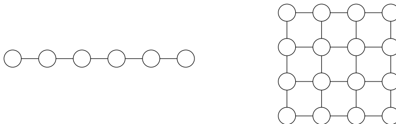
Figure 6.1: Left: chain graphs. Right: two-dimensional grid with 4-connectivity. The cut in these undirected graphs lead to Lovász extensions which are certain versions of total variations, which enforce level sets of w to be connected with respect to the graph.
