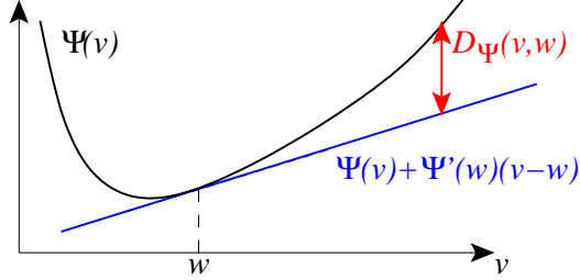
Figure 7.3: Bregman divergence: D_{\Psi}(v, w) is equal to the difference between the convex function \Psi(v) and the affine function tangent at w . When \Psi is \mu -strongly convex, then D_{\Psi}(v, w) \geq 0 with equality if and only if v = w . Moreover, we have D_{\Psi}(v, w) \geq \frac{\mu}{2}\|v - w\|^2 . Note that for a quadratic function, the Bregman divergence is a squared Euclidean norm.
