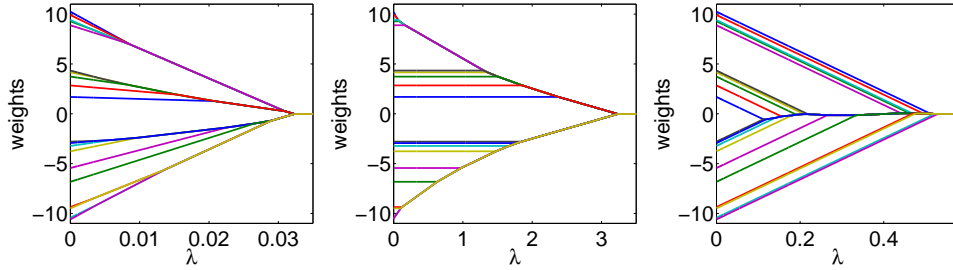
Figure 5.6: Piecewise linear regularization paths of the minimization of w \mapsto \frac{1}{2}\|w - z\|_2^2 + \lambda f(w) , for different functions of cardinality. From left to right: quadratic function (all level sets allowed), second example in §6.1 (two large level sets at the top and bottom), piecewise linear with two pieces (a single large level set in the middle). Note that in all these particular cases the regularization paths for orthogonal designs are agglomerative , while for general designs, they would still be piecewise affine but not agglomerative. For more details, see [8].
