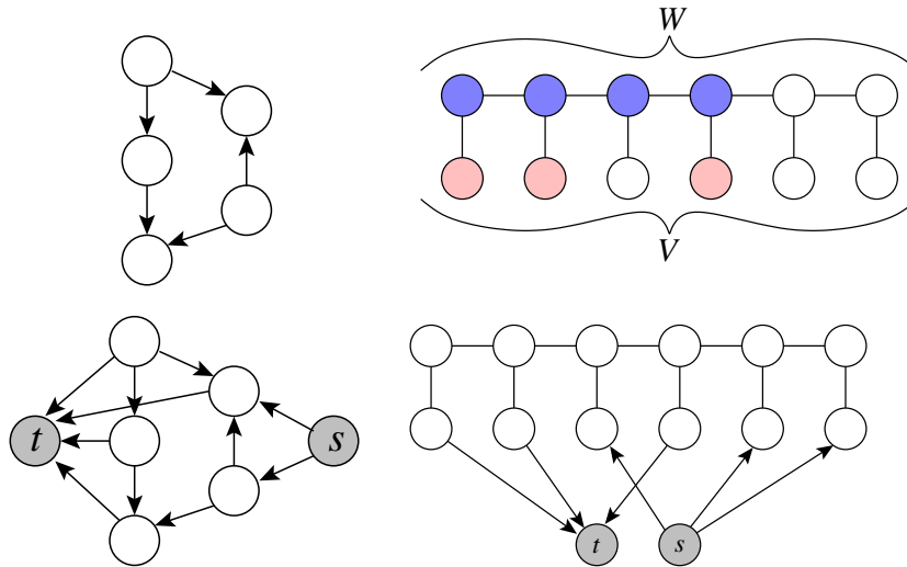
Figure 6.3: Top: directed graph (left) and undirected corresponding to regular functions (which can be obtained from cuts by partial minimization; a set A \subseteq V is displayed in red, with a set B \subseteq W with small cut but one more element than A , see text in §6.2 for details). Bottom: graphs corresponding to the min-cut formulation for minimizing the submodular function above plus a modular function (see text for details).
