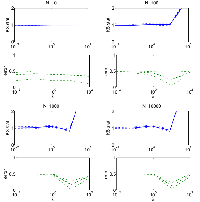
Fig. 1. Relationship between support recovery error and KS statistic as the size N of the data set increases. x-axis : regularization parameter \lambda . y-axis : KS statistic (solid line) and the support recovery error (dashed line). Thin dashed lines are error bars
